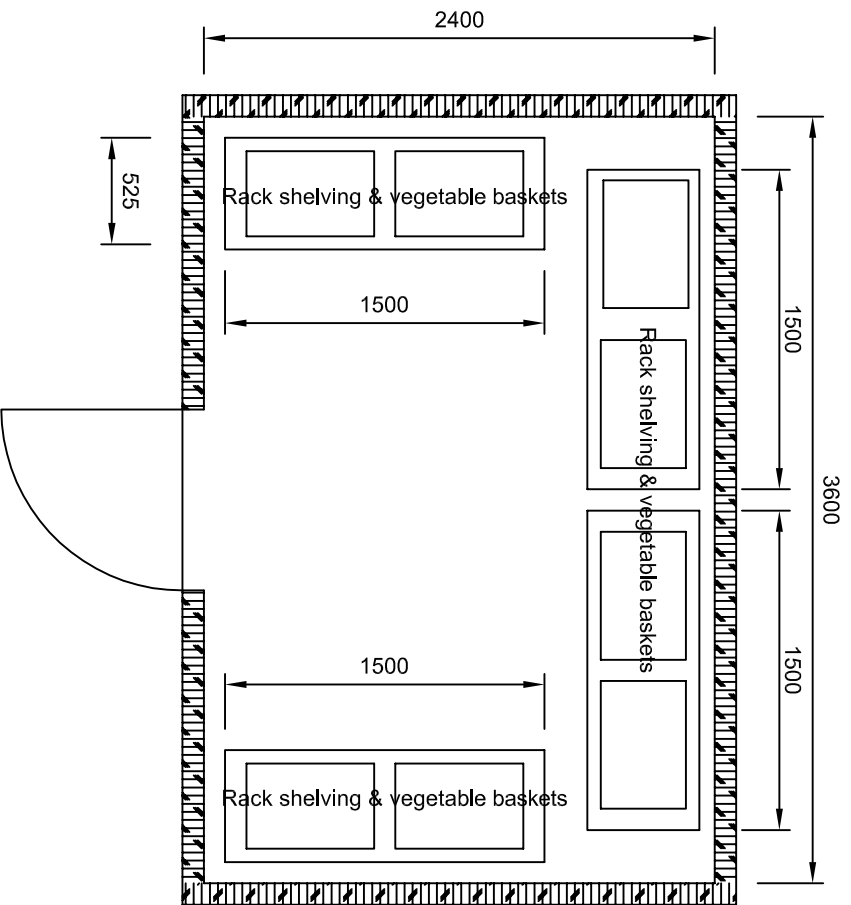
PLAN VIEW
